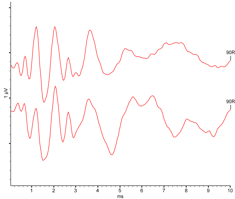
Chart 1 -- Waveforms
